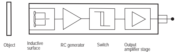
General scheme of a capacitive transducer
