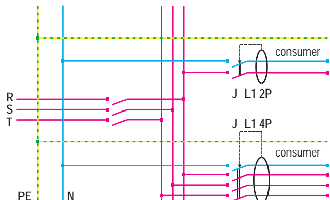
Connecting scheme
