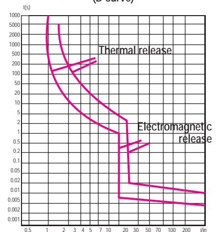
(D curve)
