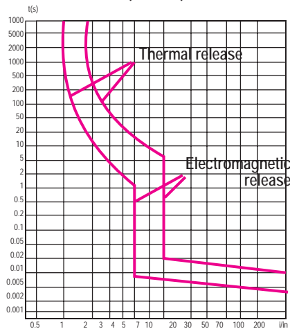
(C curve)
