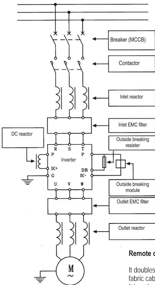
Connecting scheme of the auxiliary elements
