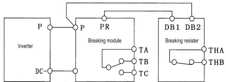
Connecting scheme of a brake resistor
